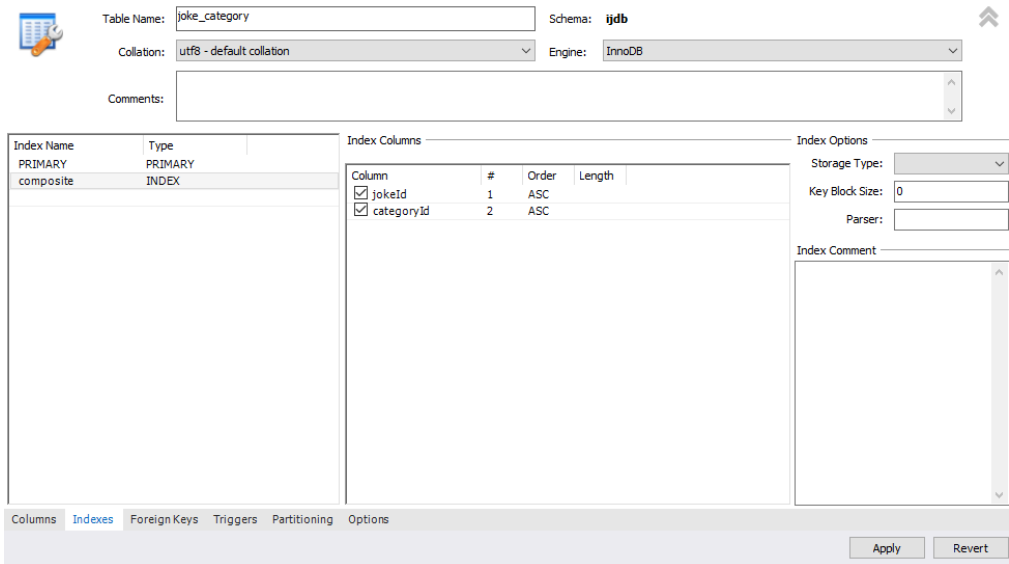
12-6. Indexes can contain multiple columns
