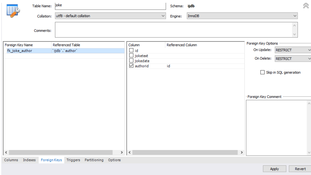
12-7. Setting up a foreign key in MySQL Workbench
