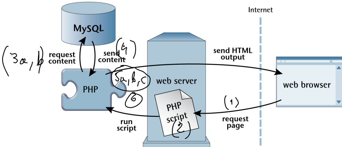
4-1. Relationships between the web server, browser, PHP and MySQL
