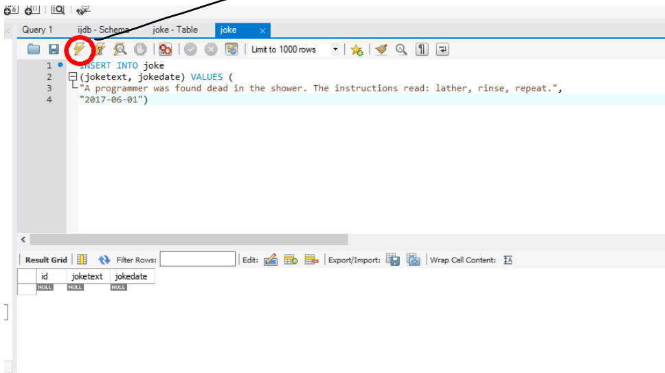
3-17. Executing an INSERT query using MySQL Workbench
